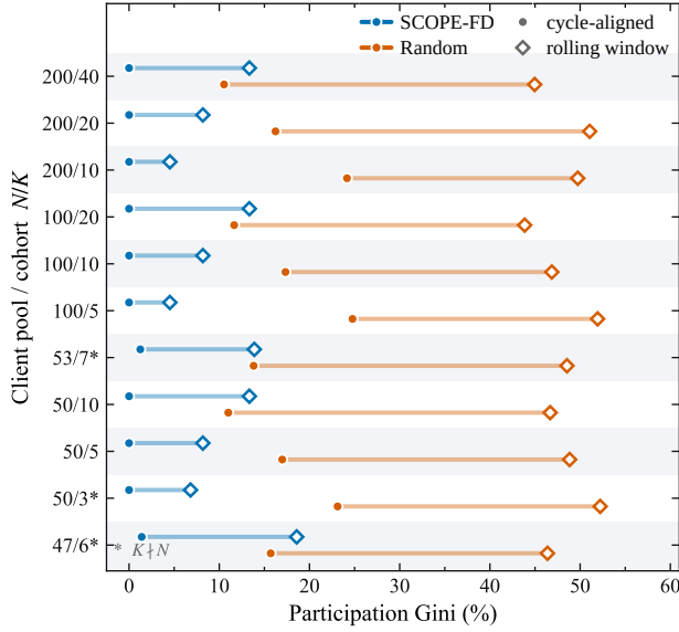
Fig. 6. Participation fairness across client-pool and cohort sizes on FMNIST over five seeds, one bar per selector. Filled circles are the cycle-aligned Gini coefficient at R = 100 ; open diamonds the rolling-window coefficient over a window offset from the participation cycle, so bar length shows how much the reading depends on window placement. Stars mark K \nmid N . Every value matches (17).
